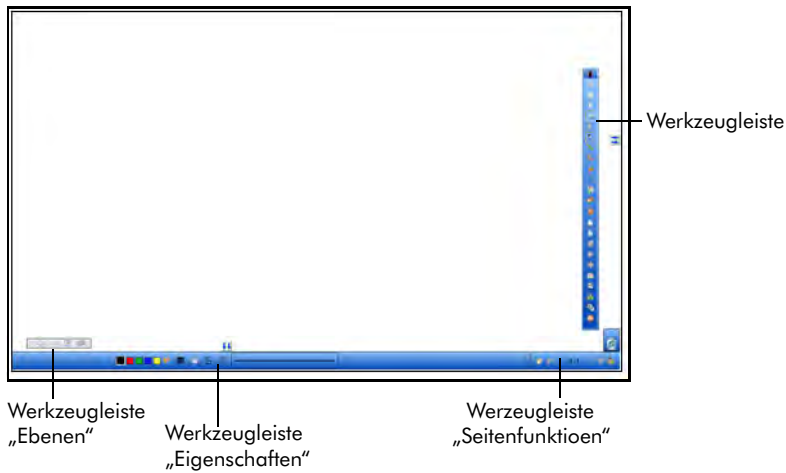
Das Workspacefenster
